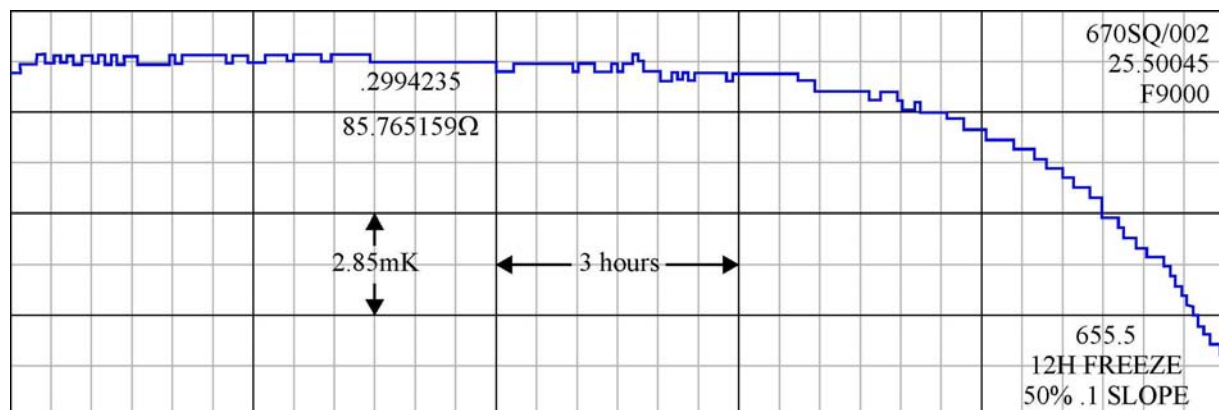
Graph 4. Pechiney 6N5 Al Freeze Curve
