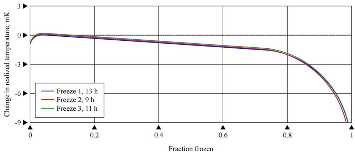
Graph 3. Pechiney 6N5 Al melt curve
