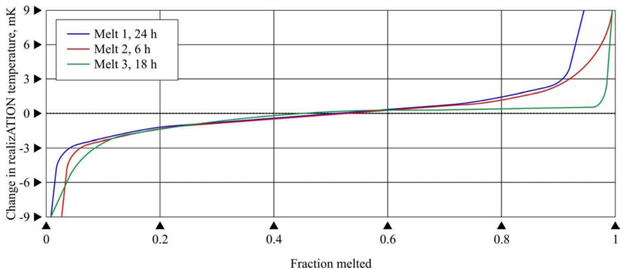
Graph 1. Melting curves for the Isotech Al fixed point cell (Isotech model ITL-M-17672-O, Serial No. Al 188)
