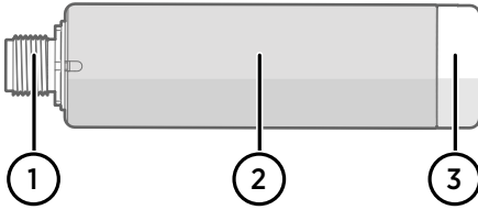
Figure 18 GMP251 probe
