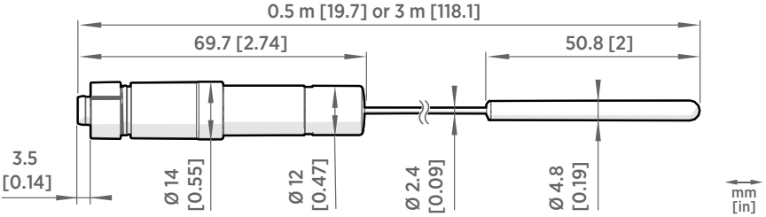
Figure 30 TMP115 probe dimensions
