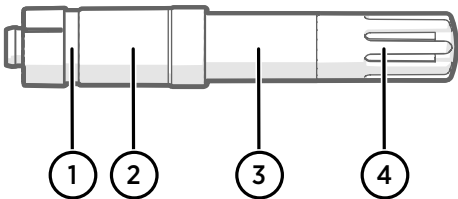
Figure 16 HMP115 probe
