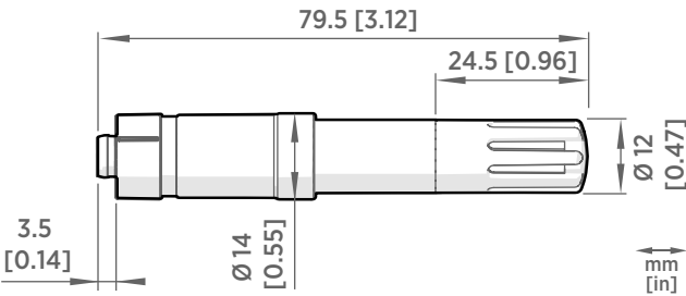
Figure 29 HMP115 probe dimensions
