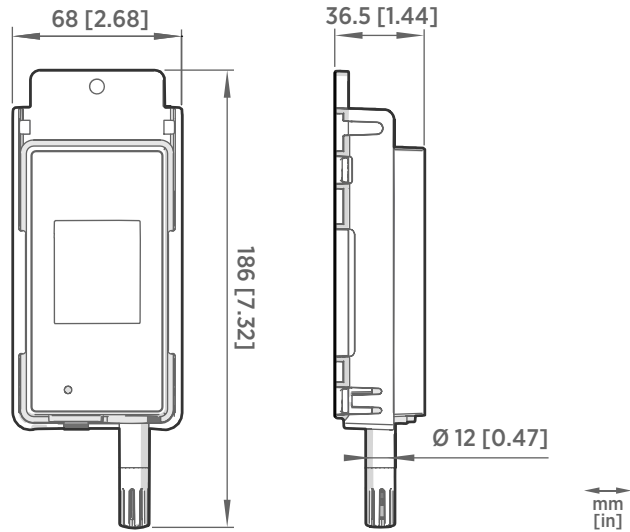
Figure 25 RFL100 dimensions with mounting bracket
