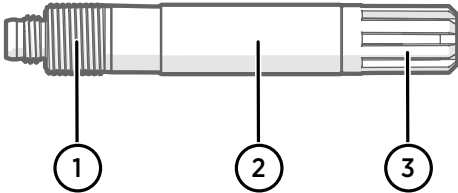
Figure 15 HMP110 probe
