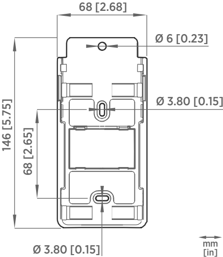
Figure 27 RFL100 mounting bracket dimensions
