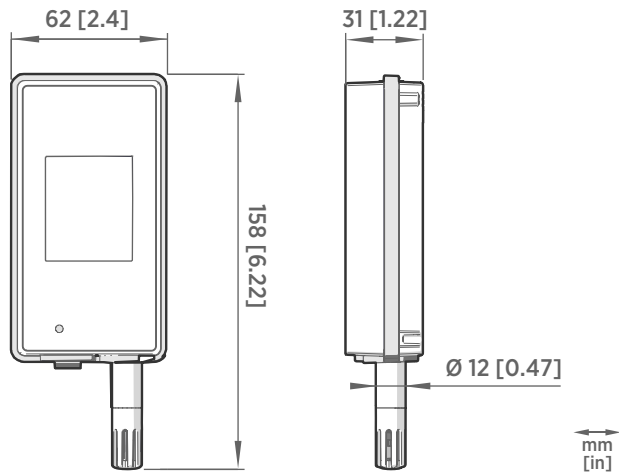
Figure 26 RFL100 dimensions without mounting bracket
