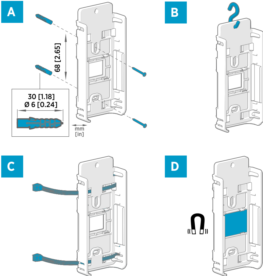
Figure 11 RFL100 mounting methods
