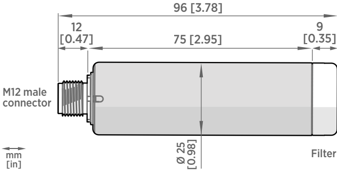
Figure 31 GMP251 probe dimensions
