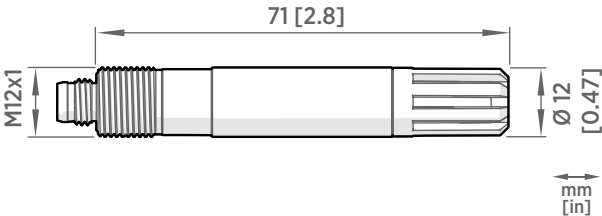
Figure 28 HMP110 probe dimensions
