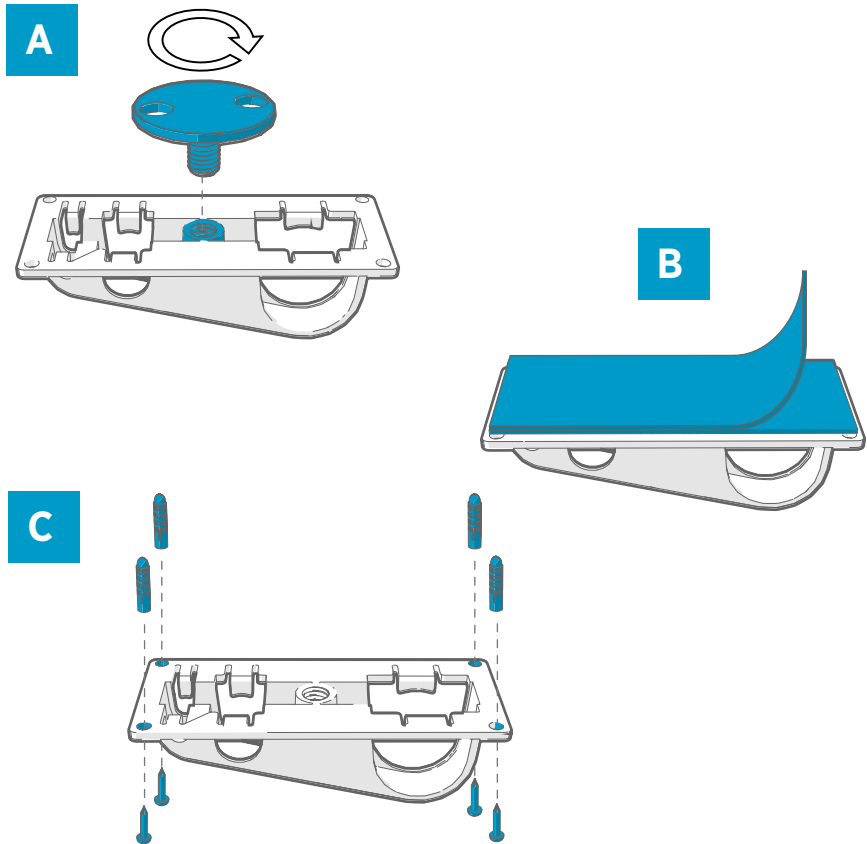
Figure 14 Probe support accessory mounting options
