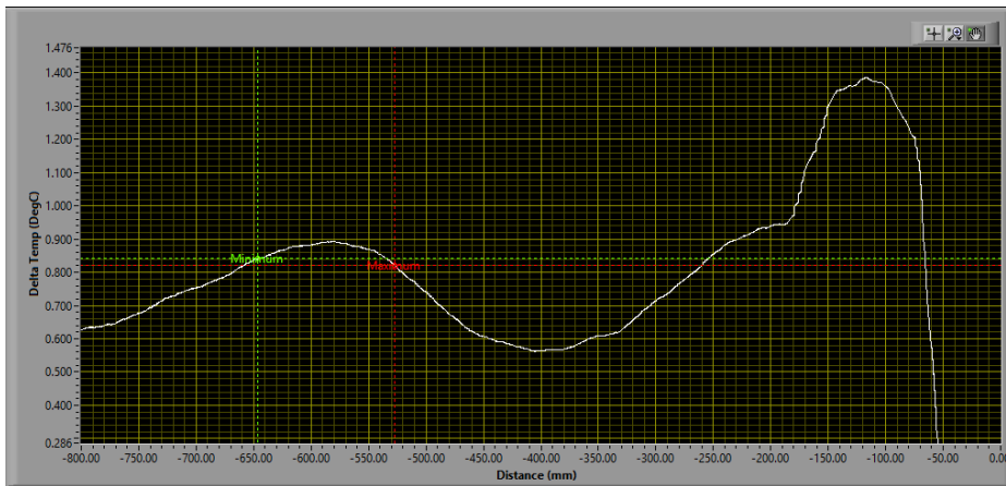
Figure 3. Scan of a Type K Thermocouple exposed over a 1 m length to a maximum temperature of 950 °C.
