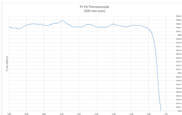
Figure 4. A scan over 500 mm of a Platinum-palladium thermocouple
