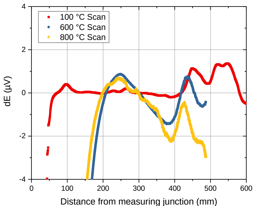
Figure 7 A graph of the homogeneity scans of the Type B thermocouple at 100 °C in the Model 881, and at 600 °C and 800 °C in the NPL homogeneity scanner.
