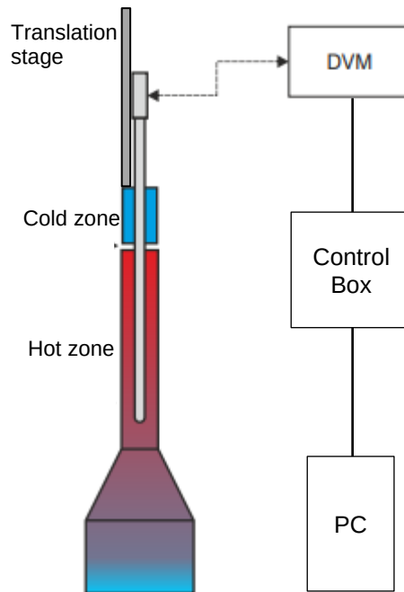
Figure 2 Isotech Homogeneity Scanner and peripheral equipment.
