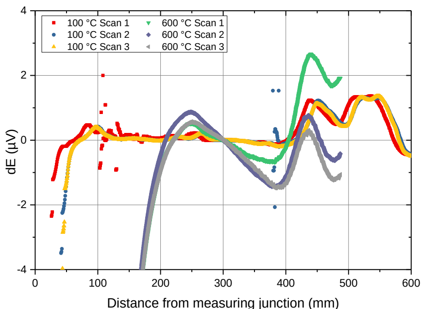
Figure 5 A graph of the homogeneity scans of the Type B thermocouple, where the x axis is the distance of the thermocouple tip from the sharp temperature gradient. The 100 °C scans were performed in the Model 881 and the 600 °C scans in the NPL scanner. The spikes seen at 100 mm and 400 mm for the scans at 100 °C are due to noise created by the thermocouple extension wires moving during the scan.
