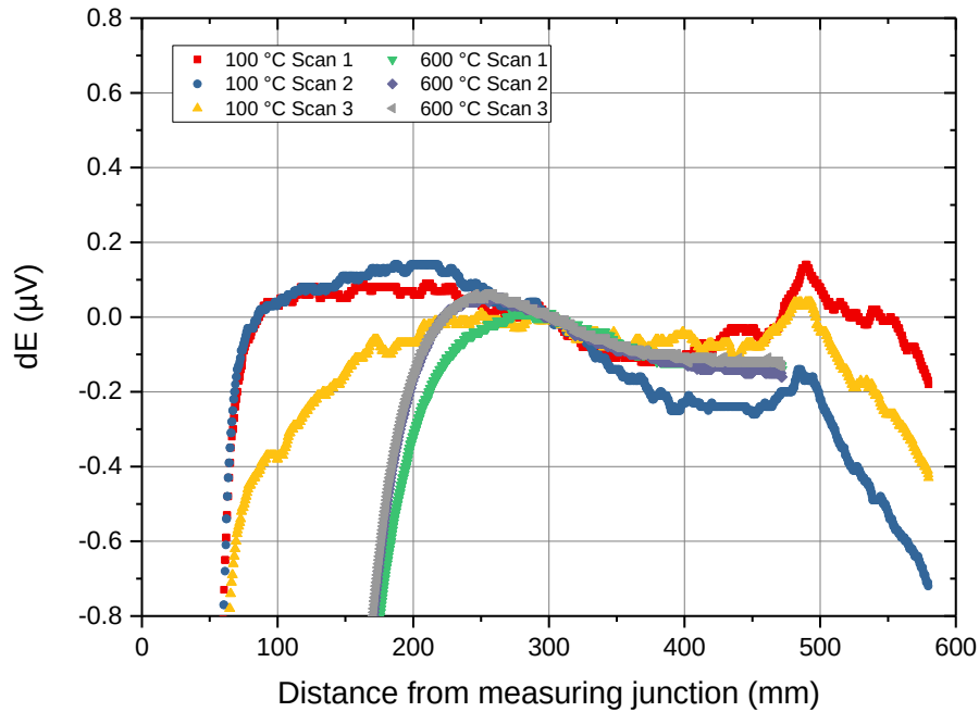
Figure 6 A graph of the homogeneity scans of the Pt-Pd thermocouple, where the x axis is the distance of the thermocouple tip from the sharp temperature gradient. The 100 °C scans were performed in the Model 881 and the 600 °C scans in the NPL scanner.
