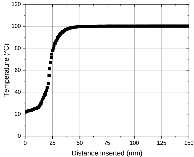
Figure 3 Graph showing the temperature gradient of the Model 881 between 0 mm insertion to 150 mm insertion. Note that the actual gradient is between 0 mm and 50 mm.
