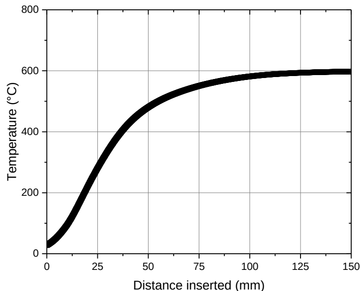
Figure 4 Graph showing the temperature gradient of the NPL scanner between 0 mm insertion to 150 mm insertion.
