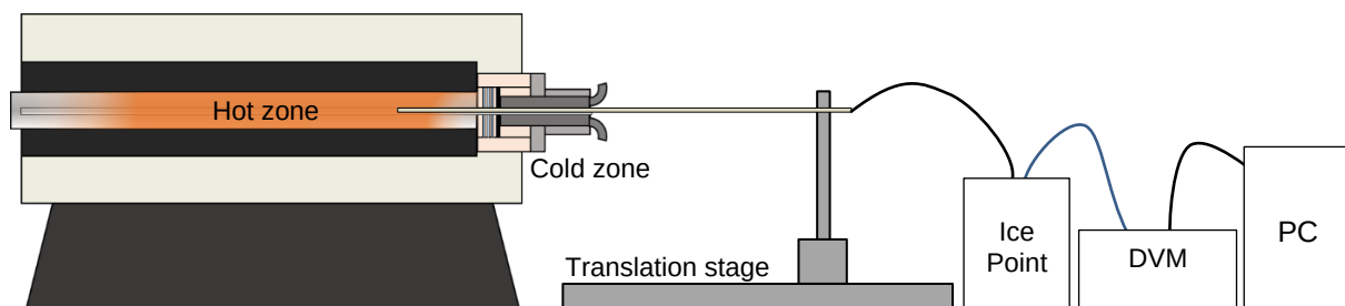
Figure 1 NPL’s homogeneity scanner and peripheral equipment.
