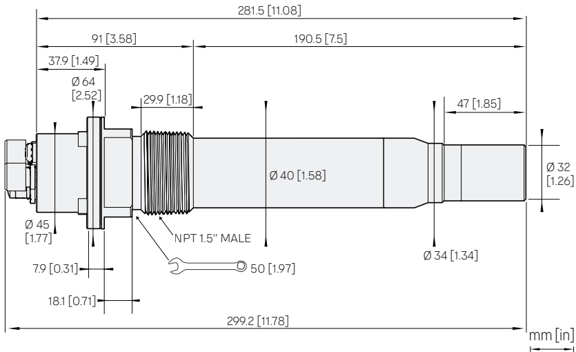
Figure 6 MGP241 dimensions
