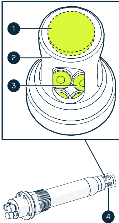
Figure 3 Probe cuvette with mirror and sensor chips
