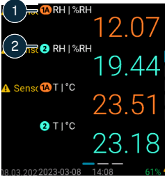
Figure 8 Measurement view showing one device connected to Indigo80 via a transmitter and the other directly to Indigo80
