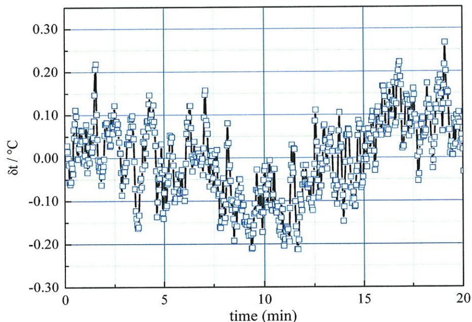
Fig. 4. Time variation of temperature at 150°C detected by a pyrometer looking into the conical part of cavity.
