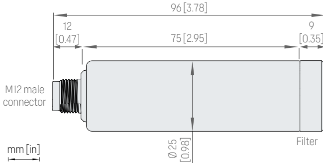
Figure 5 GMP251 dimensions
