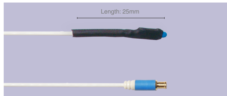
ST100B - Untipped Bare Sensor
