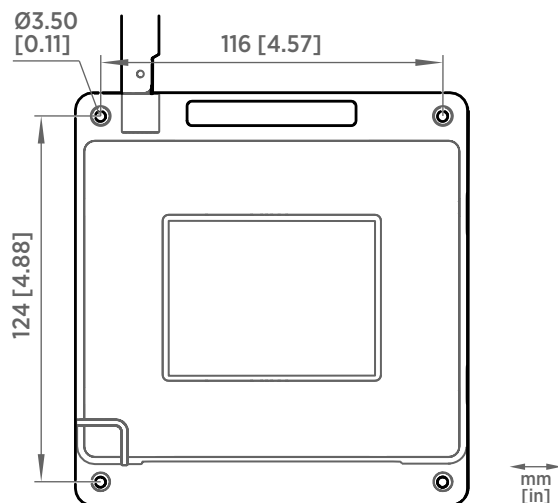
Figure 11 AP10 screw mounting dimensions
