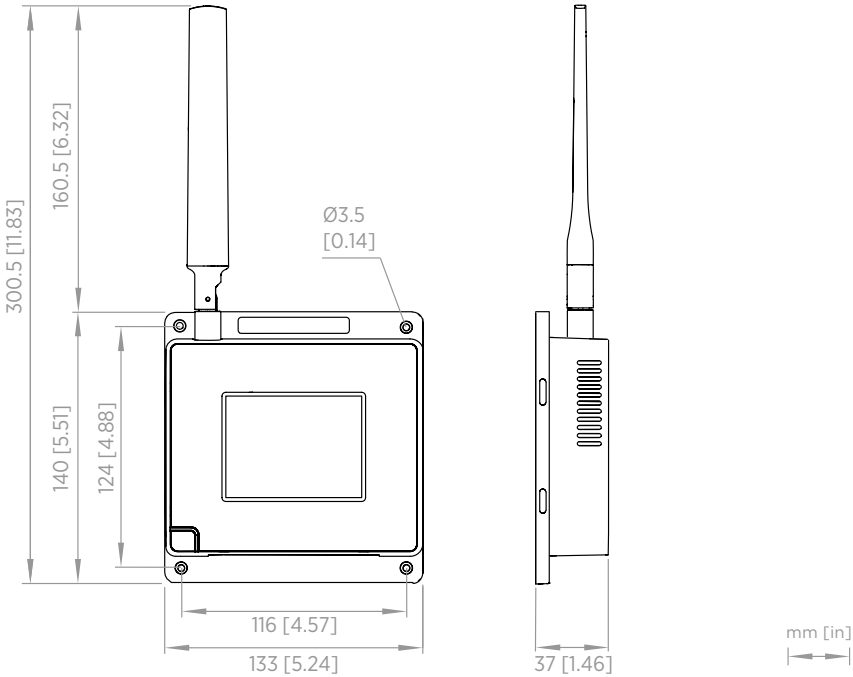
Figure 3 API0C model dimensions
