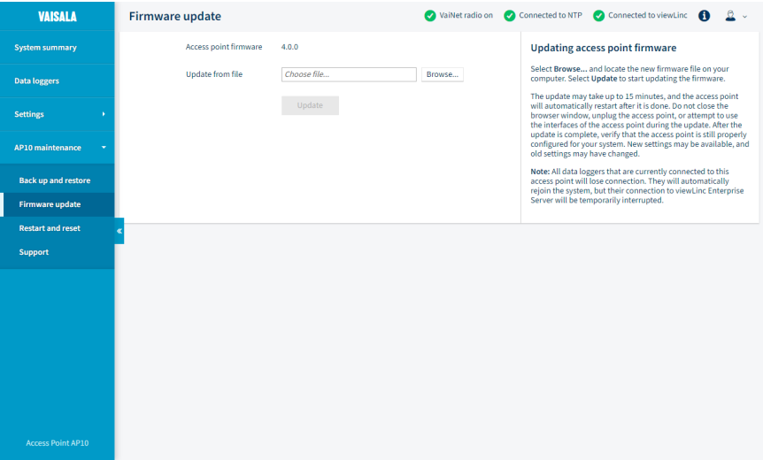
Figure 25 Web interface firmware update page
