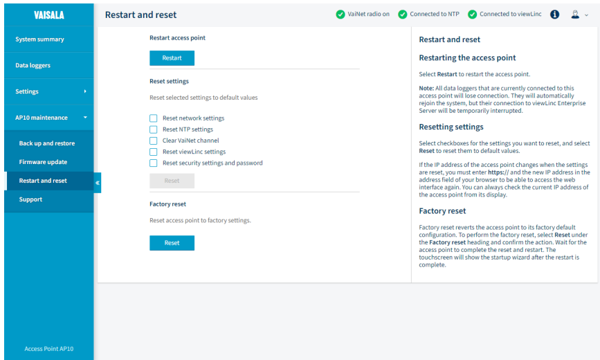
Figure 26 Web interface restart and reset page
