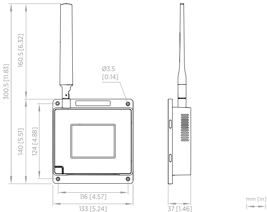
Figure 31 AP10C model dimensions
