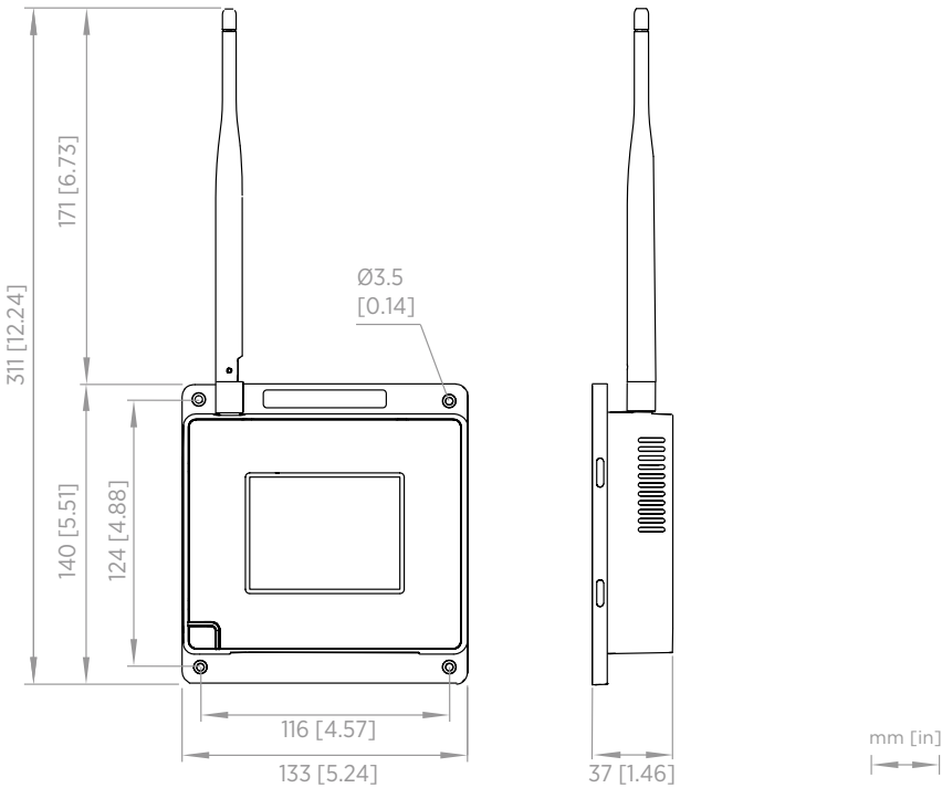
Figure 30 AP10 access point dimensions
