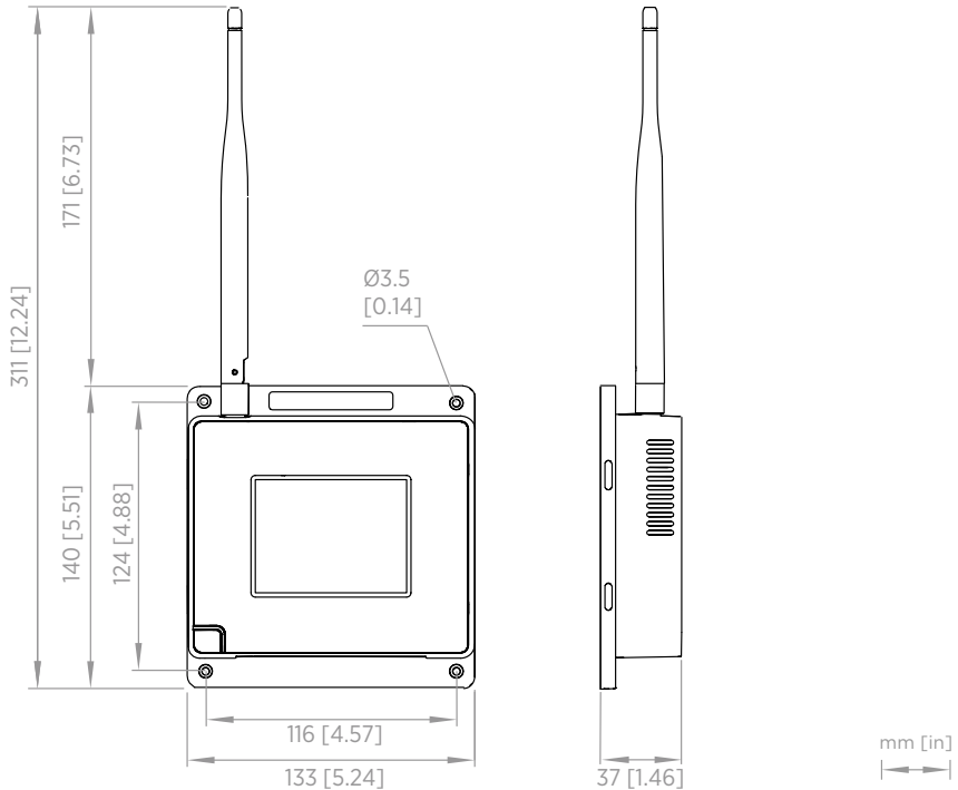
Figure 2 AP10 access point dimensions
