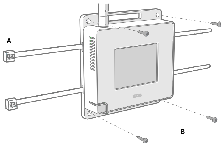
Figure 10 AP10 mounting methods
