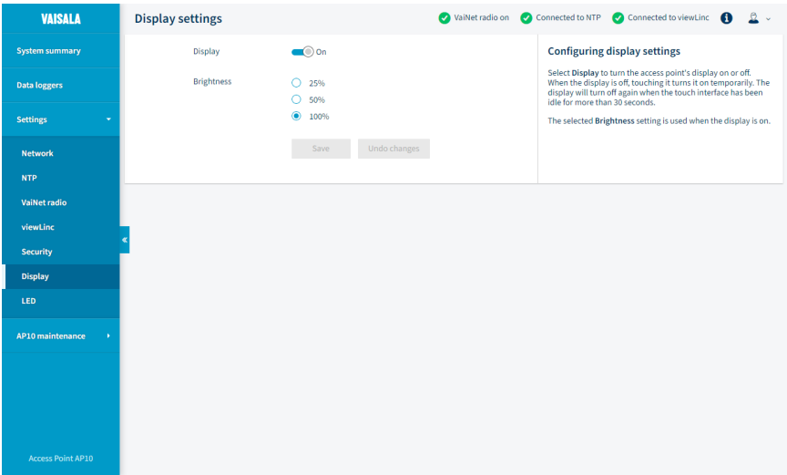
Figure 22 Web interface display settings page
