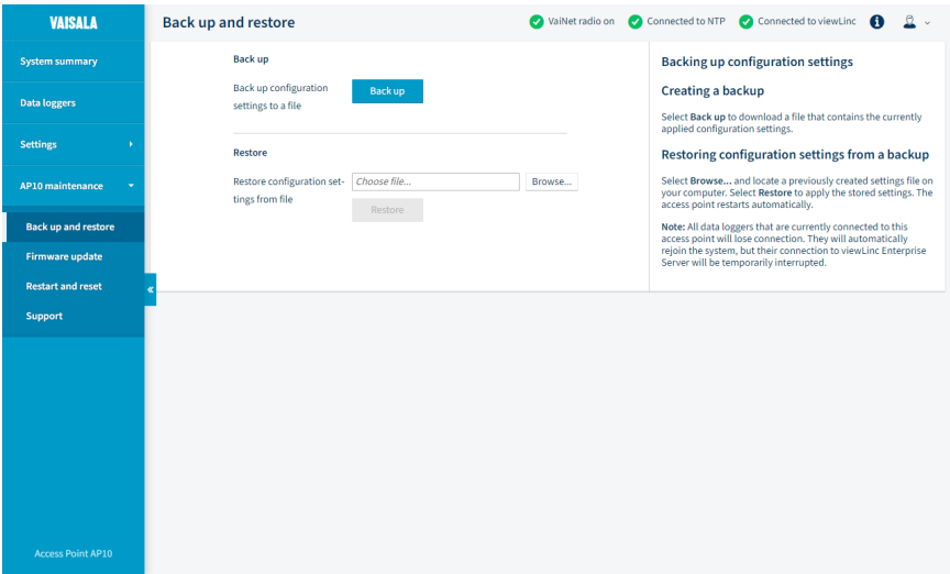
Figure 24 Web interface backup and restore page
